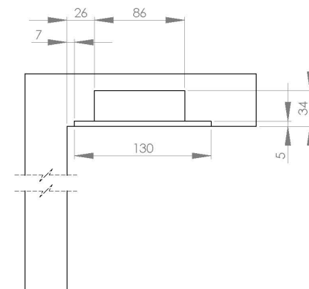
FRAME ELEVATION MORTISE DETAIL
