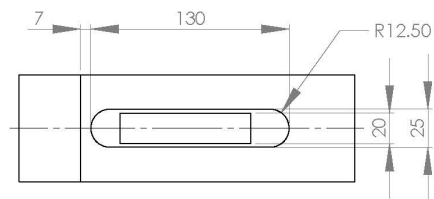
UNDERSIDE OF FRAME MORTISE DETAIL
