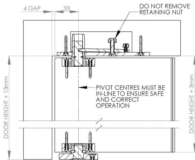
TYPICAL DOOR/FRAME SECTION
