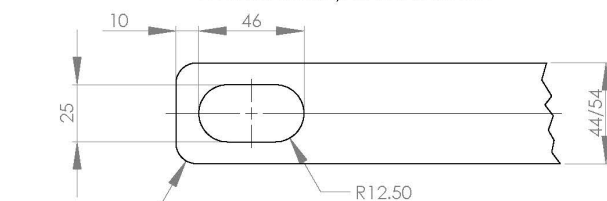
TYPICAL DOOR LEAF DETAILS BOTH ENDS
